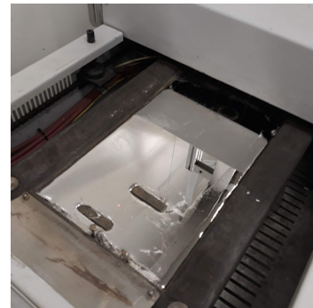
Solder pot post cleaning. Shiny with no evidence of dross.
