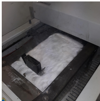
A thin layer of 5744 placed on top of solder pot surface.
