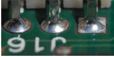
Figure 5. Top side joints
