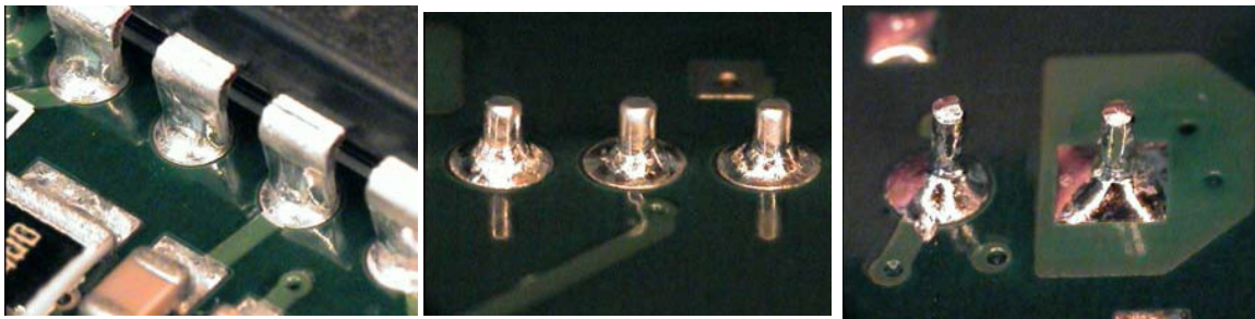
Figure 7. Various through-hole parts showing excellent wetting on top and bottom-side
