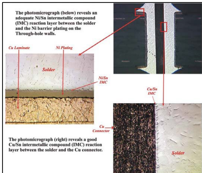
Figure 10. Cross-sectional tests wave soldered through-hole
